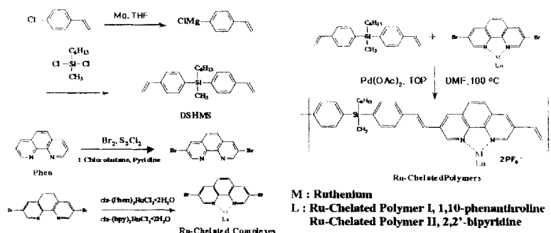
SCHEME 1 Synthetic routes to the monomers and the silicon-based copolymers with Ru(II)-chelated complexes.
